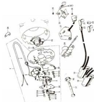
15. Contact Breaker
